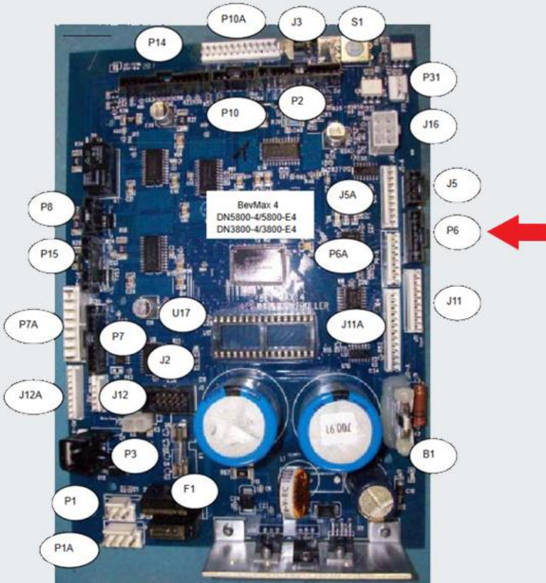
Above: Diagram of MDB/EXE Controller Connections- BevMax4: DN 5800-4, DN 3800-4, DN 5800-E4, DN 3800-E4
